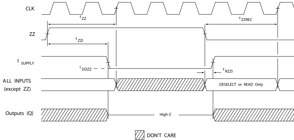
Figure 8. ZZ Mode Timing [20, 21]
