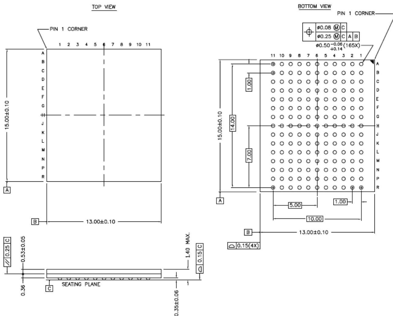
Figure 11. 165-Ball FBGA (13 x 15 x 1.4 mm)
